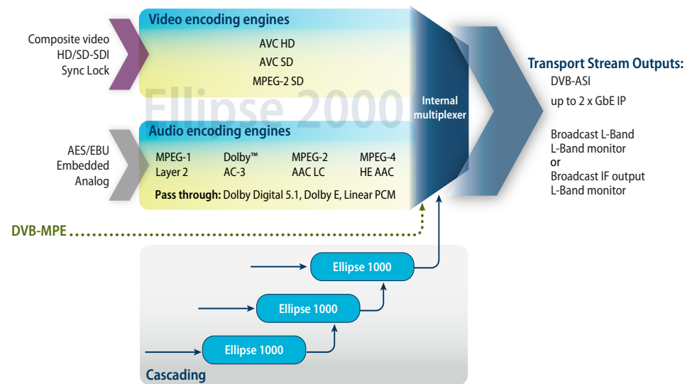
Ellipse 2000 block diagram
