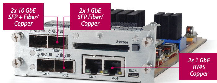
The optional Quad GbE I/O module in ProStream 9100 with ACE delivers up to 2 Gb of IP throughput.
